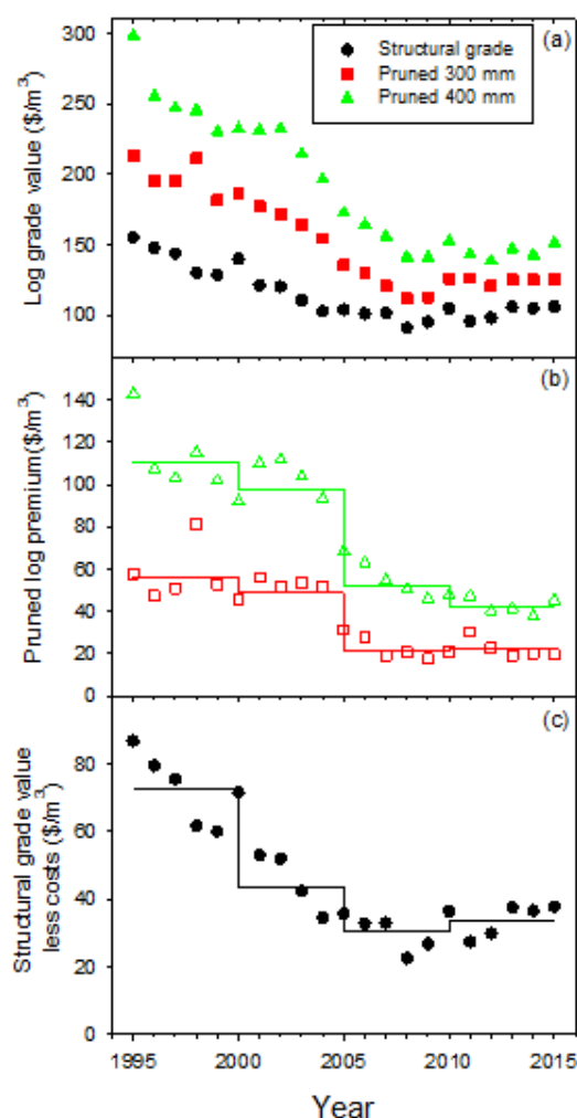
Figure 1. Variation in (a) real (inflation adjusted) log grade value, (b) real pruned log premium for P30 and P40 and (c) real net structural grade value from 1995 to 2015. Horizontal lines drawn through the data in figures (b) and (c) represent averages from 1995-2000; 2001-2005; 2006-2010 and 2011-2015.
