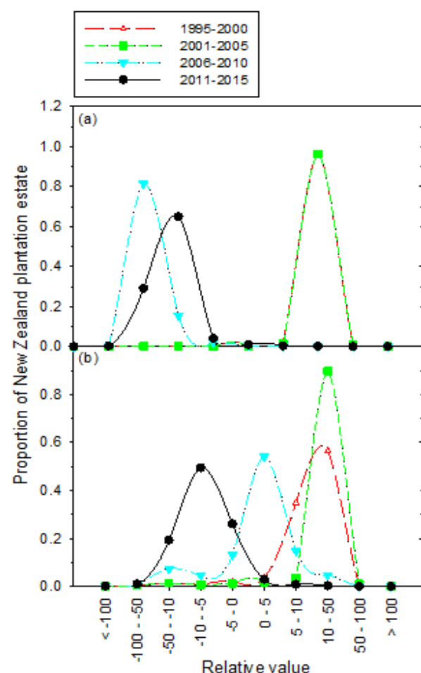
Figure 3. The distribution of relative value (net value of a clearwood regime/net value of a structural grade regime) for the New Zealand plantation estate from 1995-2000, 2001-2005, 2006-2010 and 2011-2015 for (a) P30 and (b) P40.
