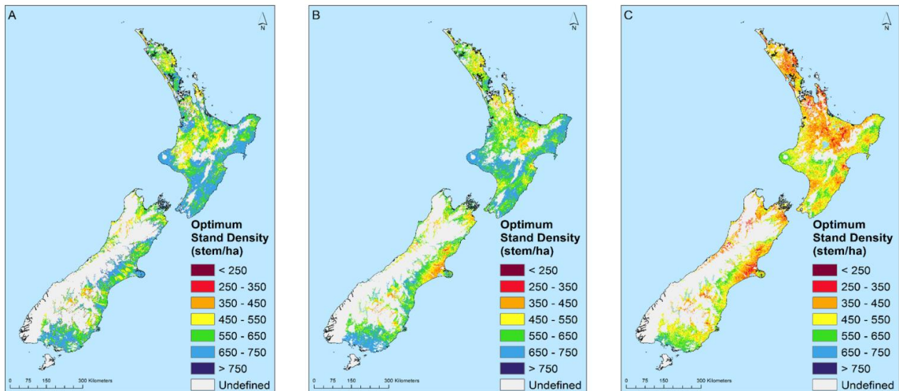
Figure 2. Spatial variation in optimal stand density for (a) S30, (b) P30 and (c) P40. Surfaces were generated using values of pruned log premium and net structural grade value that were averaged from 1995-2015.
