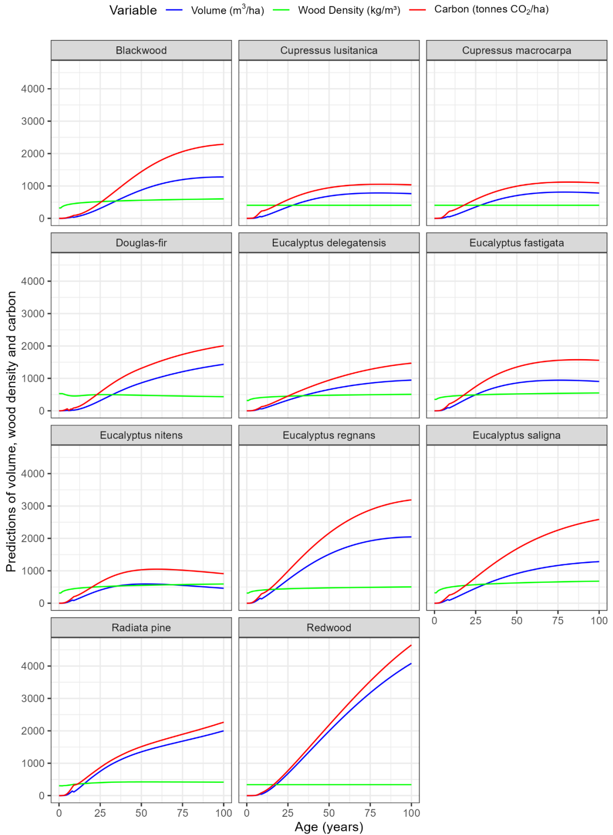
Appendix Figure 2. Predictions of total volume (blue line), wood density (green line) and total carbon (red line) against age, by species. Model predictions were extracted from the calculator using the North Island productivity indices shown in Table 1 (Appendix). All runs had a starting stand density of 1,000 stems/ha and were thinned at age 9 to 500 stems/ha. The values of volume and carbon were reduced by 15% to account for stand gaps.
